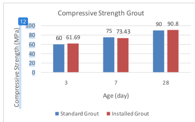
Figure 6. Compressive strength Grout
