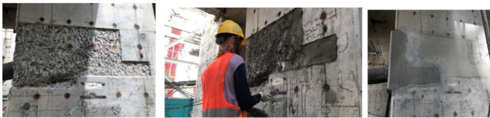
Figure 2. Honeycomb from 10 mm up to 10 mm upto less than 50 mm and concrete cover less than 40 mm
