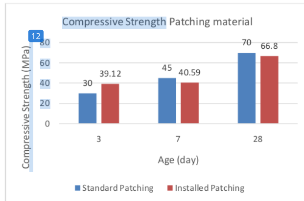
Figure 7. Compressive strength patching material
