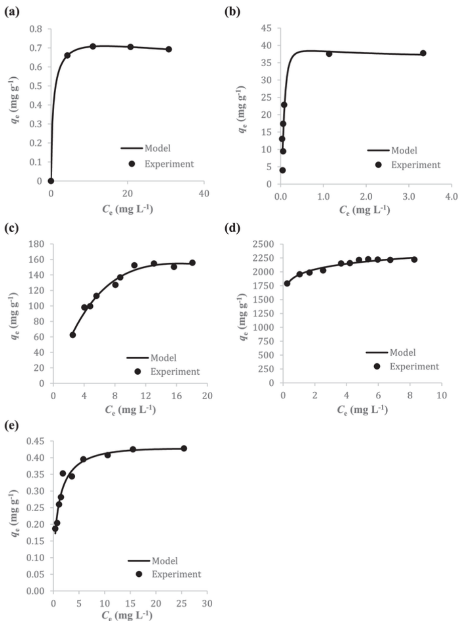
Fig. 2. Curve of plotting q_e versus C_e for assessing the behaviors of AgNPs adsorption on (a) GB, (b) AIOMP, (c) FPC, (d) PFC and (e) AP by the Fritz-Schlunder isotherm model.
