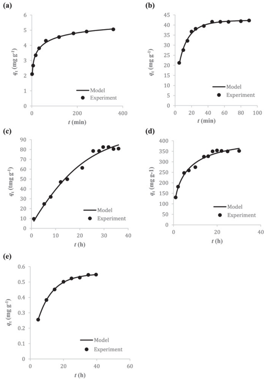
Fig. 1. Curve of plotting q_t versus t for assessing the behaviors of AgNPs adsorption on (a) GB, (b) AIOMP, (c) FPC, (d) PFC and (e) AP by the fractal-like mixed 1, 2-order kinetic model.
