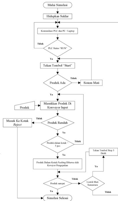
Gambar 8. Diagram alir simulator
