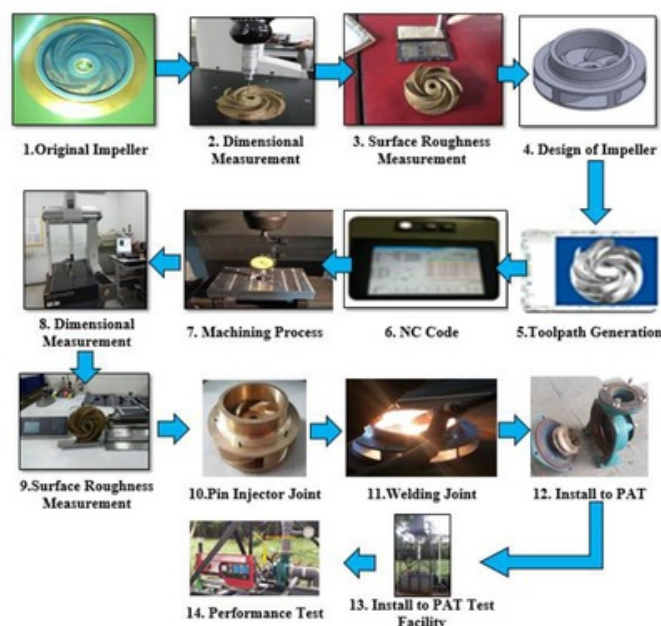
Fig.1. Manufacturing process of machined centrifugal impeller
