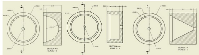
Figure 2 Possible shapes of the cavity: half ball (B3, B5, B8), tube (T3, T5, T8) and cone (K3, K5, K8)
