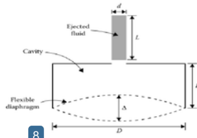
Figure 9 Stroke length on a synthetic jet
