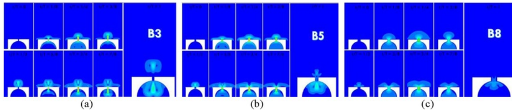
Figure 10 The formation process of vortex rings in condition: (a) B3; (b) B5; and (c) B8
