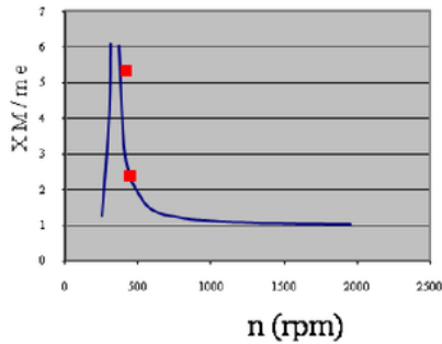
Fig.6. Change of MX/me vs n ; M = 40 (kg)
