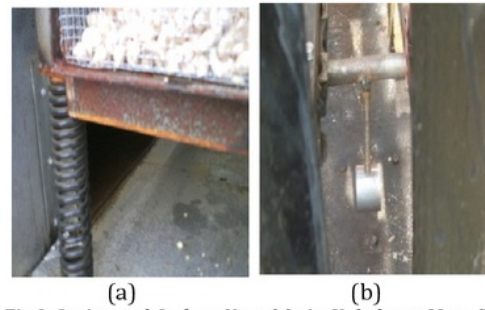
Fig.3. Spring and Cashew Nuts (a); An Unbalance Mass (b)
