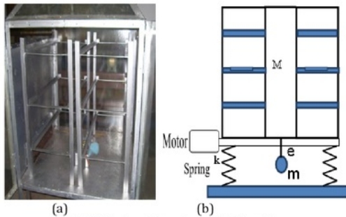
Fig.2. Drying Chamber (a); Vibration Components (b)
