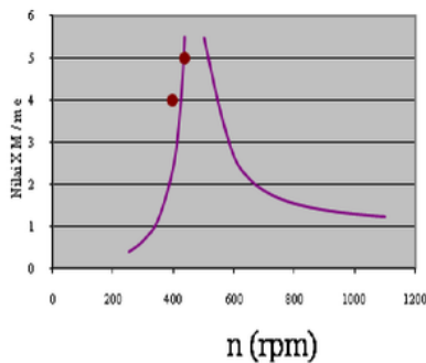
Fig.7. Change of MX/me vs n ; M = 20 (kg)
