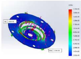
Gambar 11. Static strain
