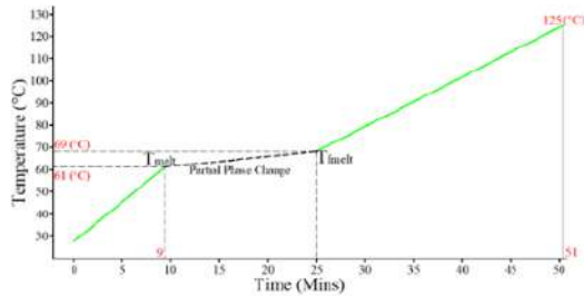
Figure 3. Charging for hybrid PCM (90% paraffin and 10% volcanic ash)
