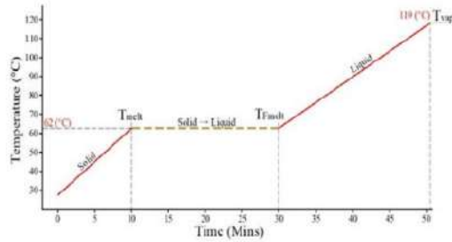
Figure 1. Charging for pure paraffin
