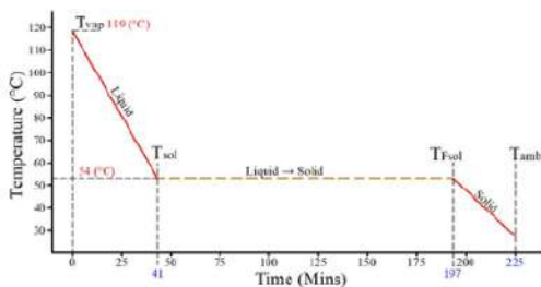
Figure 2. Discharging for pure paraffin
