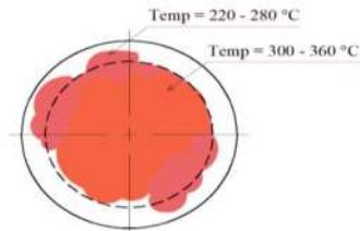
FIGURE 9. THE ABSORBED HEAT ON THE RECEIVER SURFACE AT A POSITION ABOVE THE FOCAL POINT
