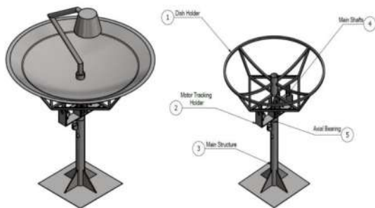
FIGURE 1. THE PROPOSED NEW DESIGN FOR IIR PARABOLIC DISH
