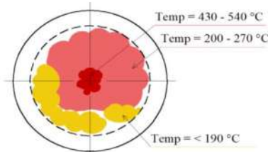
FIGURE 7. THE ABSORBED HEAT ON THE RECEIVER SURFACE AT POSITION EXACT THE FOCAL POINT
