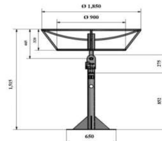
FIGURE 2. STRUCTURAL GEOMETRY FOR THE NEW DESIGN FOR IIR PARABOLIC DISH SYSTEM
