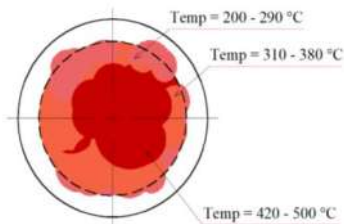
FIGURE 8. THE ABSORBED HEAT ON THE RECEIVER SURFACE AT A POSITION BENEATH THE FOCAL POINT
