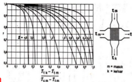
Figure 8: Correction Factor to Counterflow LMTD for Crossflow Heat Exchanger, Both Fluids Unmixed, One Tube Pass.
