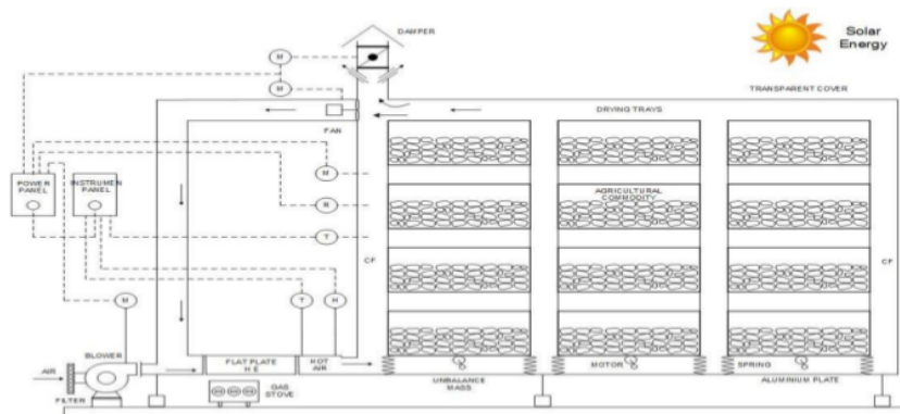
Figure 1: An Environmentally Friendly Drying Machine that uses Vibration Components and Gas Fuel.
