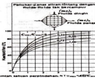
1 Figure 4: Heat-Exchanger Effectiveness for Crossflow with Both Fluids Unmixed.
