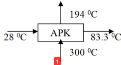
Figure 7: Temperature on Shell and Tube Heat Exchanger.
