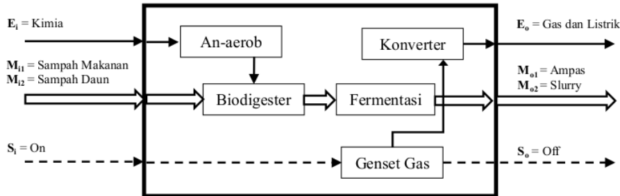
Gambar 6. Diagram fungsi biodigester tipe fixed dome
