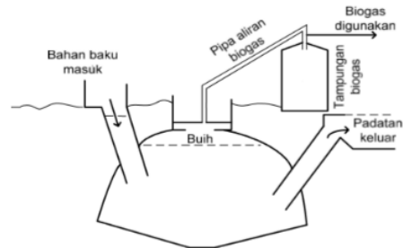
Gambar 1. Biodigester tipe fixed dome [6]
