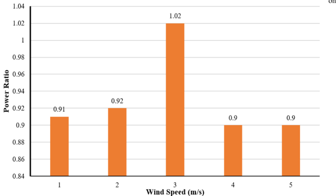
Fig. 7: Experimental result for power ratio at pitch 3D
