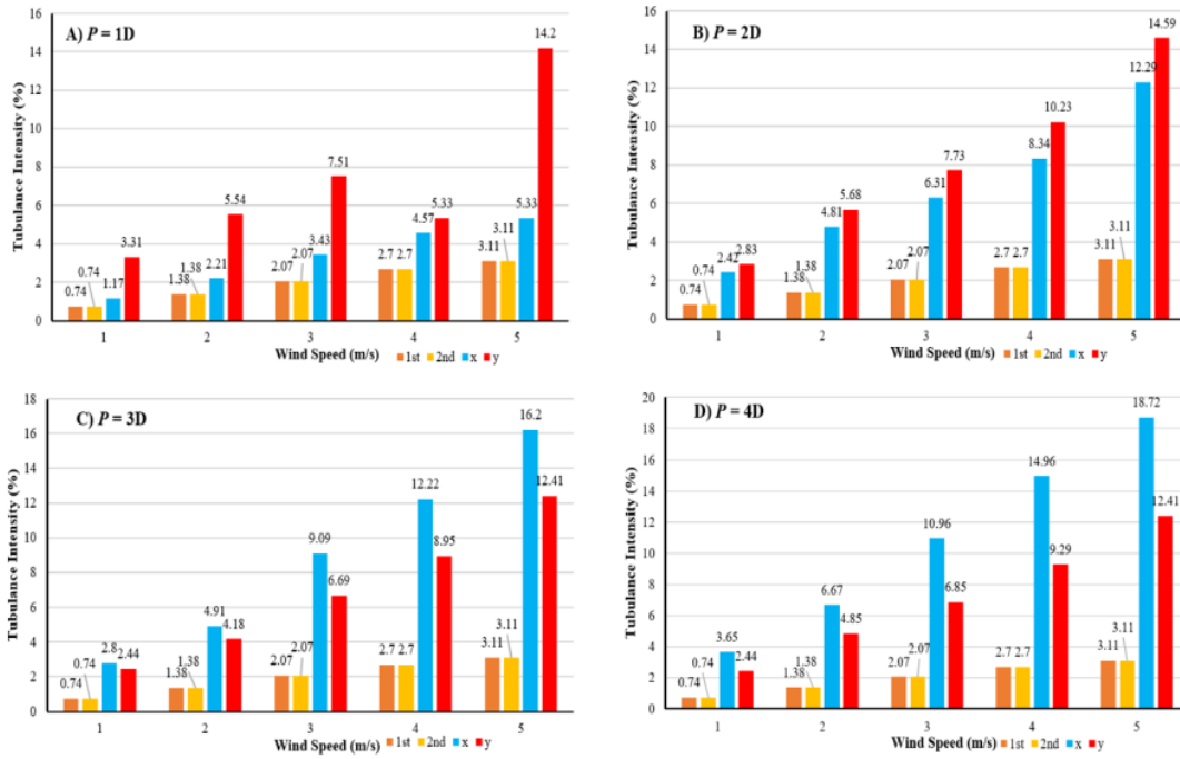
Fig. 4: Turbulence value at different configuration
