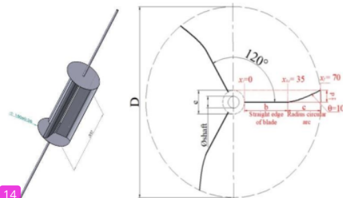
14 Fig. 1: The geometry of the Savonius turbine
