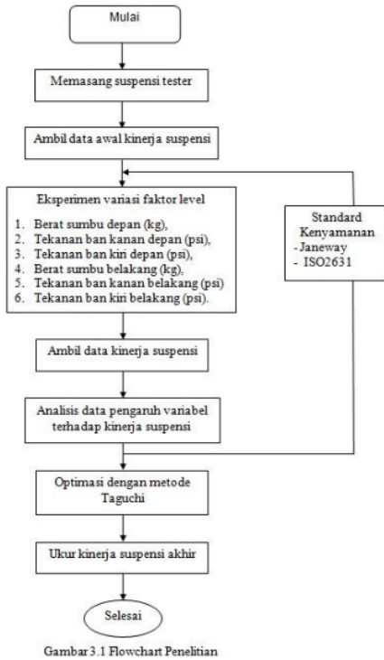
Gambar 3.1 Flowchart Penelitian
