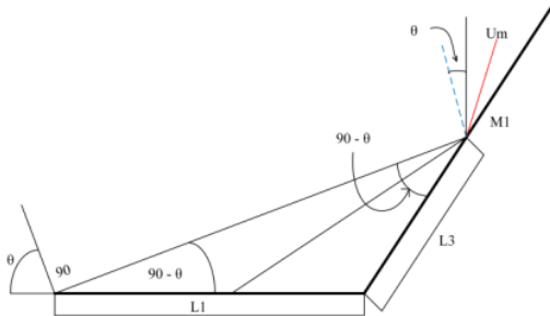
Fig. 5. The triangle geometry of the CPV system
