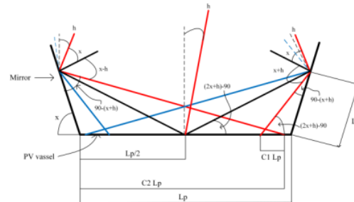
Fig. 3. The direction of irradiation sunlight to the PV module-reflective mirror
