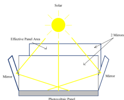
Fig. 1. PV module – 4 mirror systems
