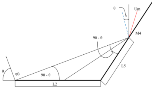
Fig. 6. The triangle geometry of the CPV system
