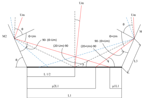
Fig. 4. The geometry model used for CPV systems
