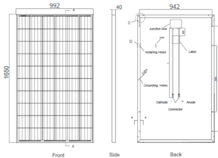
Fig. 7. Dimension of PV module system
