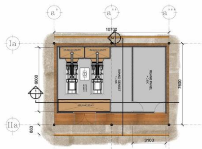
DENAH RUANG GENSET
